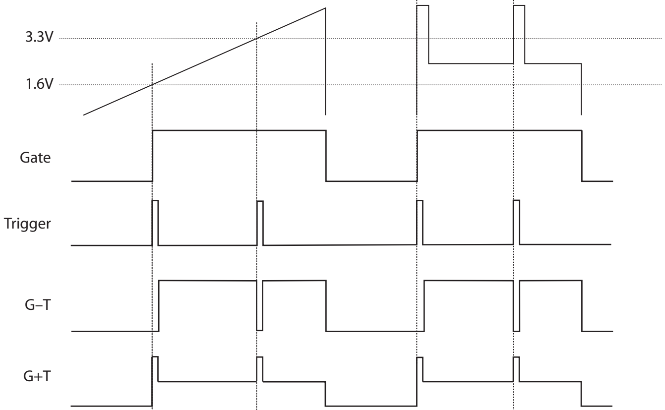
Analogue Waveform
